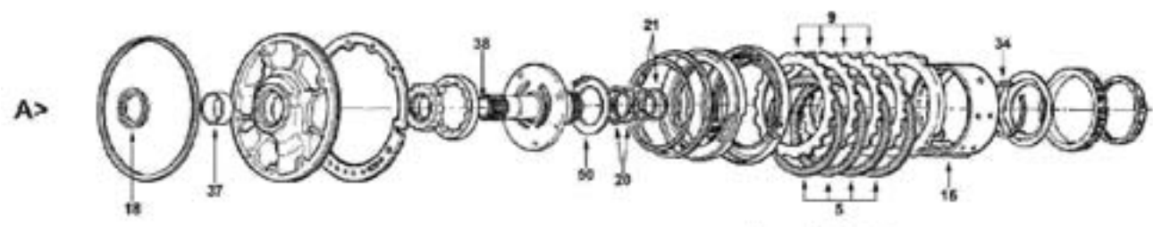
Intermediate Clutch
